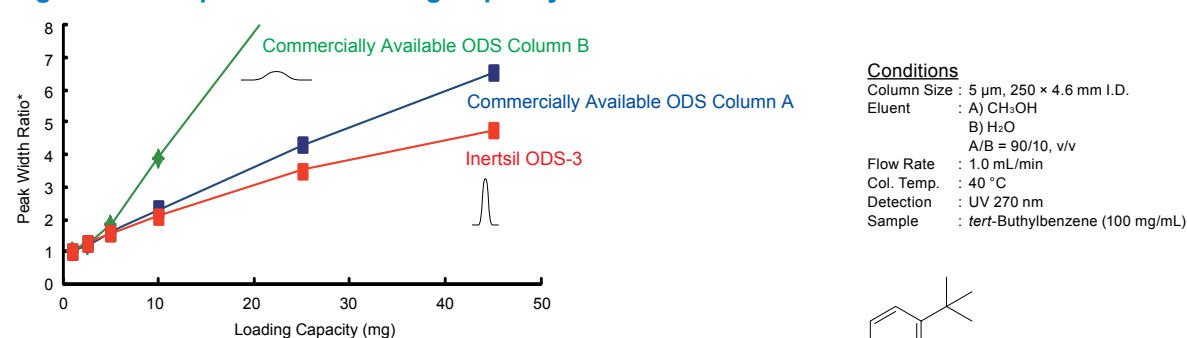
Figure 2 : Comparison of Loading Capacity
