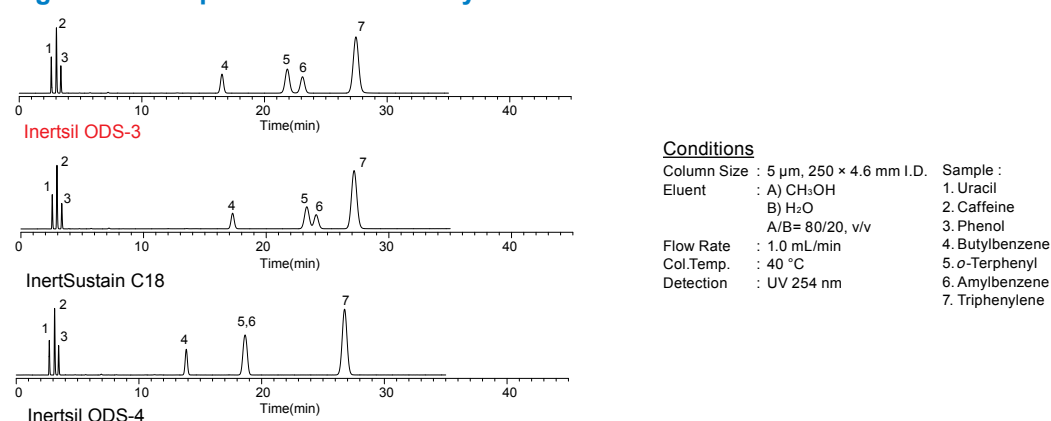
Figure 1 : Comparison of Retentivity
